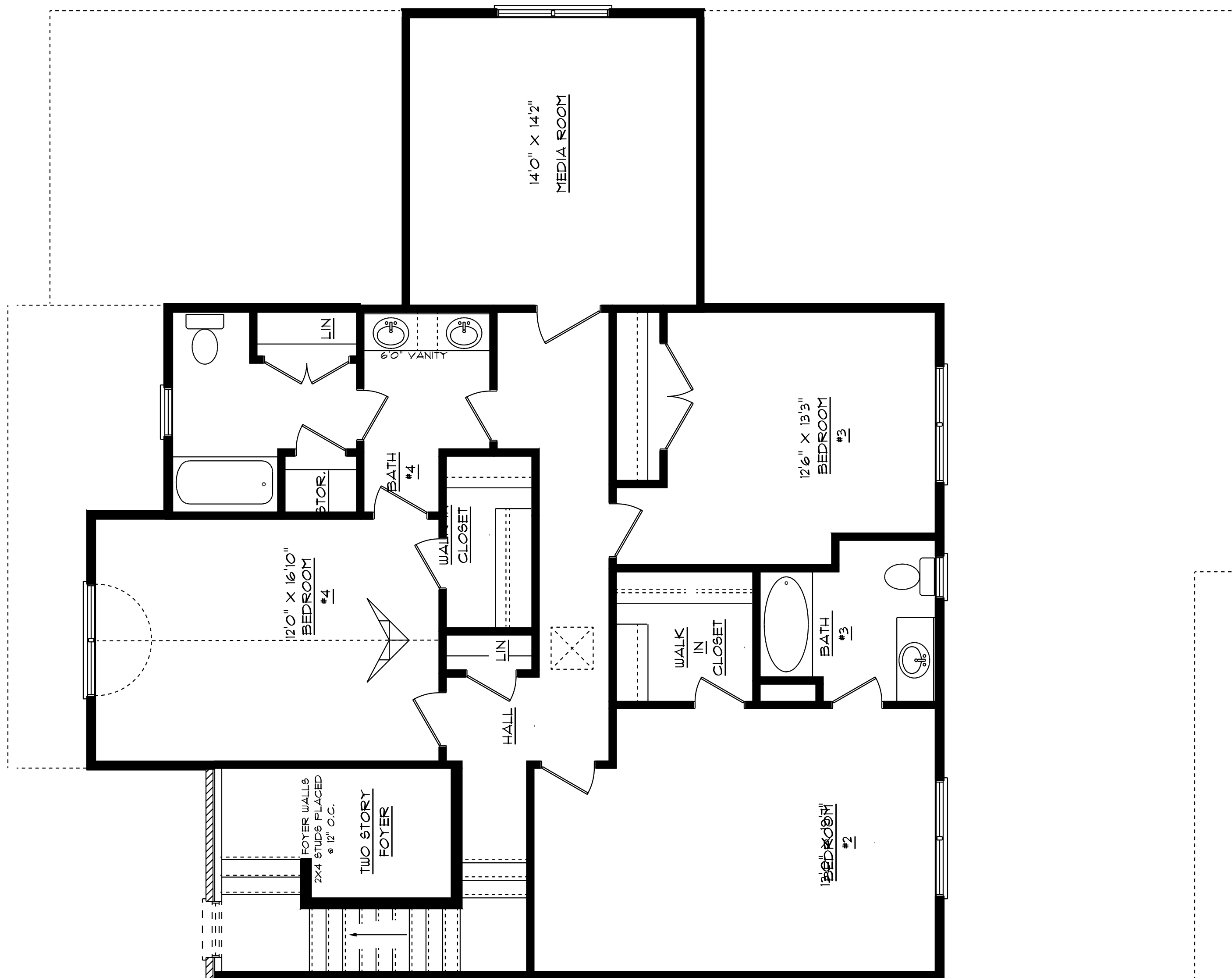
SECOND FLOOR PLAN 1290 S.F. SECOND FLOOR (DOES NOT INCLUDE TWO STORY FOYER) 8'0" CEILING HEIGHT 6" WINDOW HEADER HEIGHT
